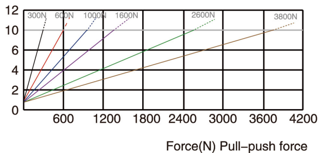
Speed ( mm/s )
