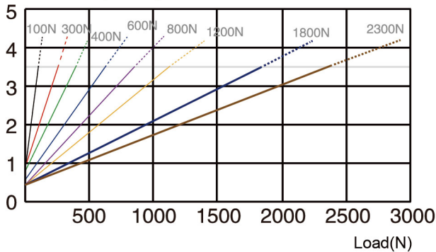
Speed(mm/s)
