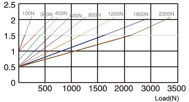
Current(A) ( 24V )
