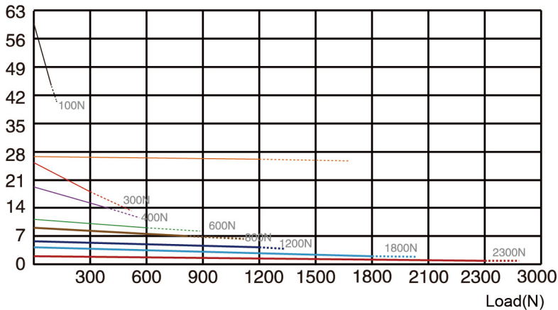
Speed(mm/s)
