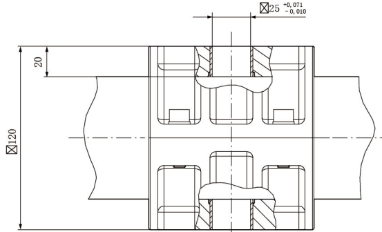
Trunnion 25mm casing pipe
