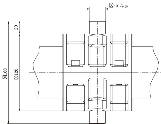
Trunnion 25mm pin
