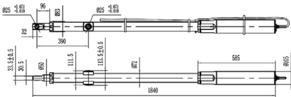
Main linear actuator
