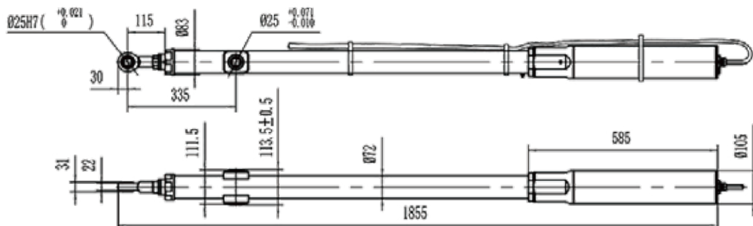
Minor linear actuator
