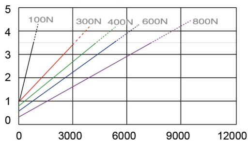
Current A(12VDC)
