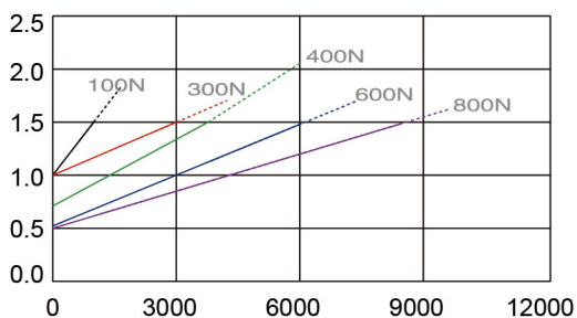
Current A(24VDC)
