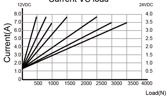
Current VS load
